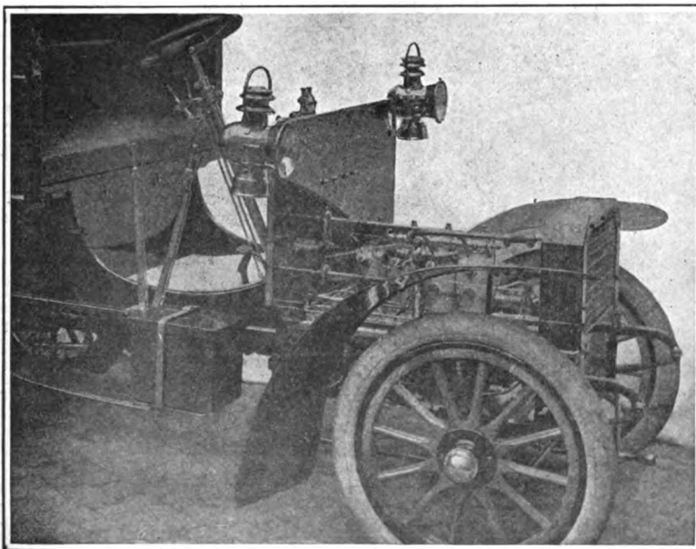
ENGINE AND CONTROL MECHANISM OF HUMBER THREE-PASSE GER CAR.
